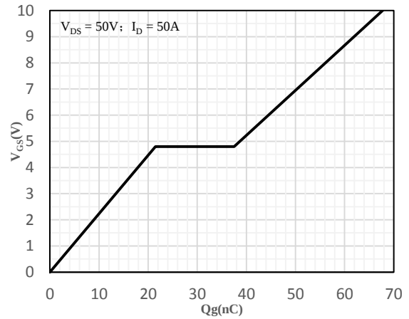
Fig 10 Gate-Charge Characteristics
